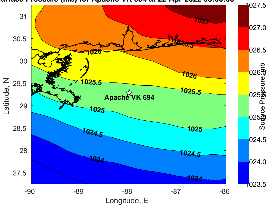
Surface Pressure (mb) for Apache VK 694 at 22-Apr-2022 03:00:00
